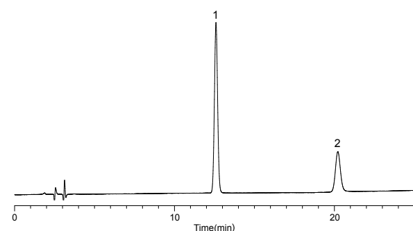
Figure 1 : Crospovidone
