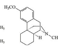
3:Dextromethorphan (Basicity)
