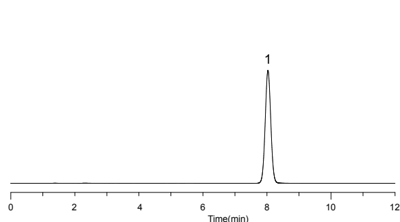
Figure 2: Voriconazole
