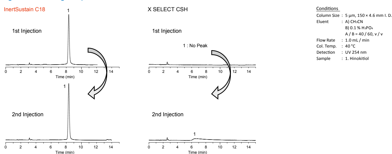
Figure 3 : Chelating Compounds
